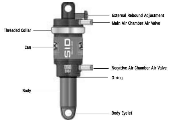
SID Rear Shock
