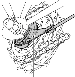
Cassette joint
