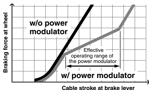
Braking Performance Comparison
